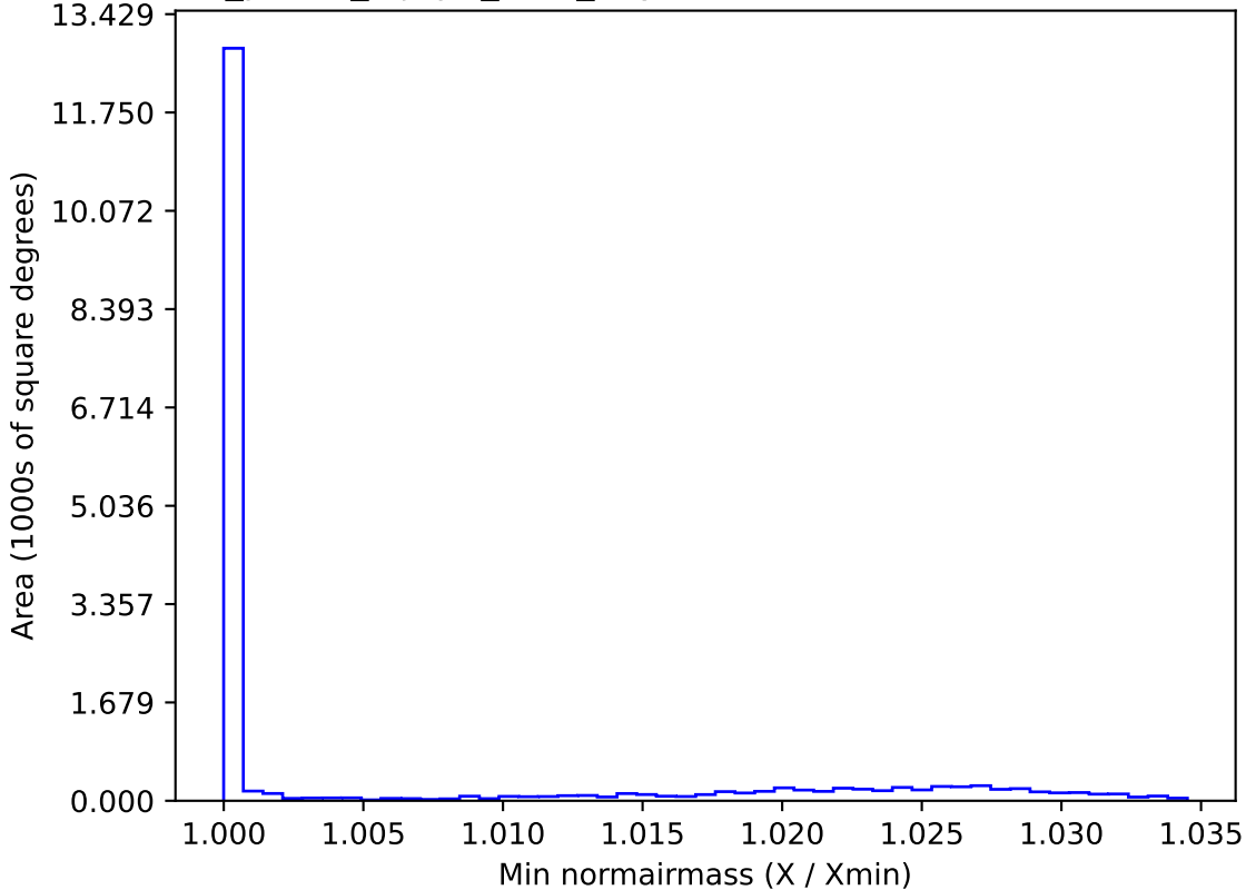
roll_pause_mjdp0_v3.4_10yrs WFD i band: Min normairmass
