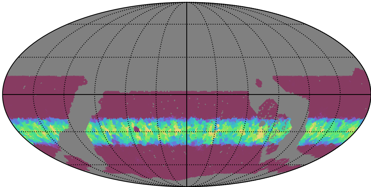
roll_pause_mjdp0_v3.4_10yrs WFD g band: Min normairmass
