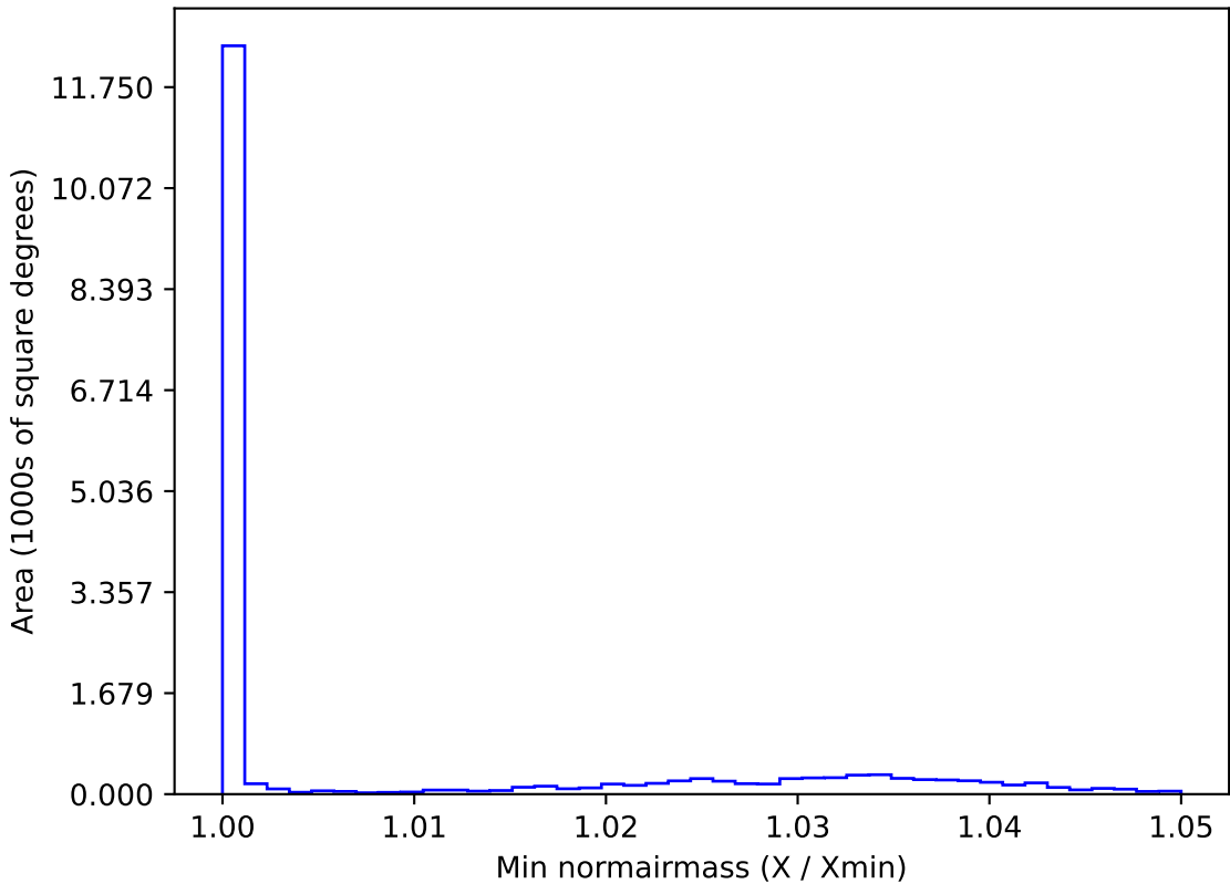
roll_pause_mjdp0_v3.4_10yrs WFD g band: Min normairmass
