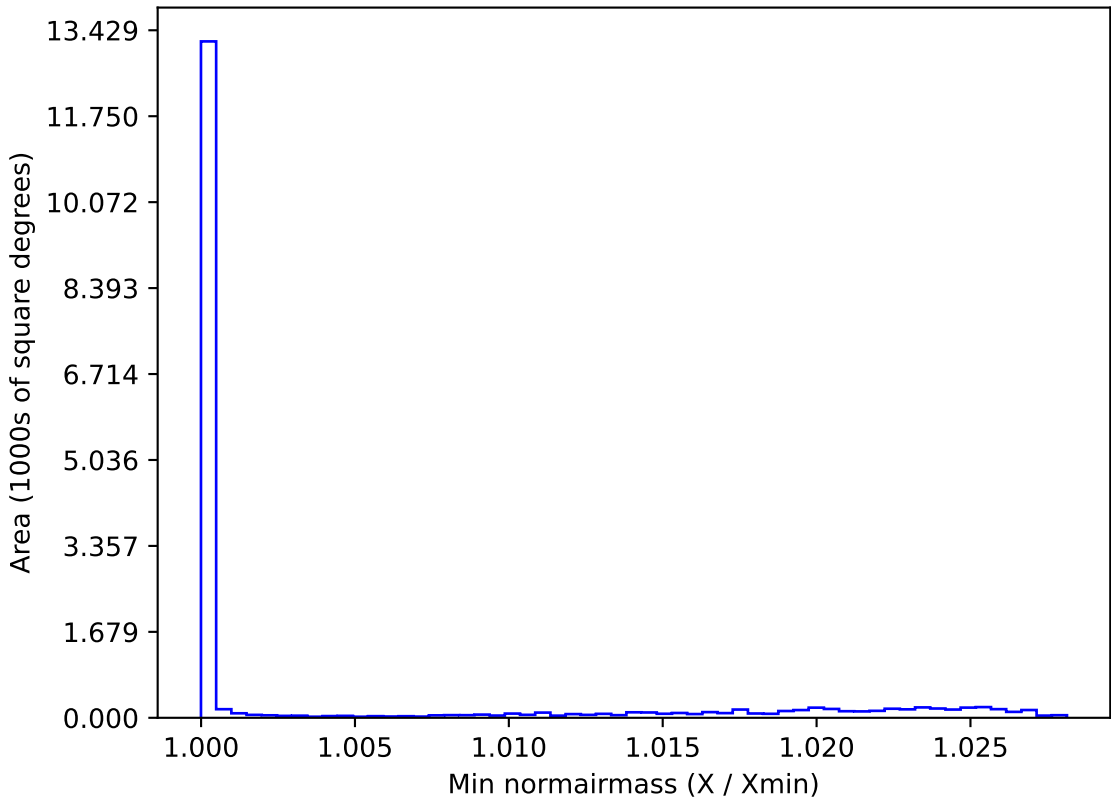
roll_pause_mjdp0_v3.4_10yrs WFD all bands: Min normairmass
