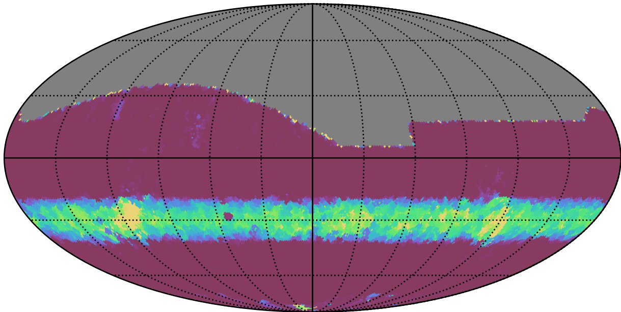
roll_pause_mjdp0_v3.4_10yrs All sky z band: Min normairmass
