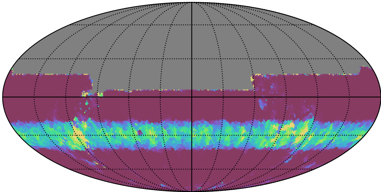
roll_pause_mjdp0_v3.4_10yrs All sky u band: Min normairmass
