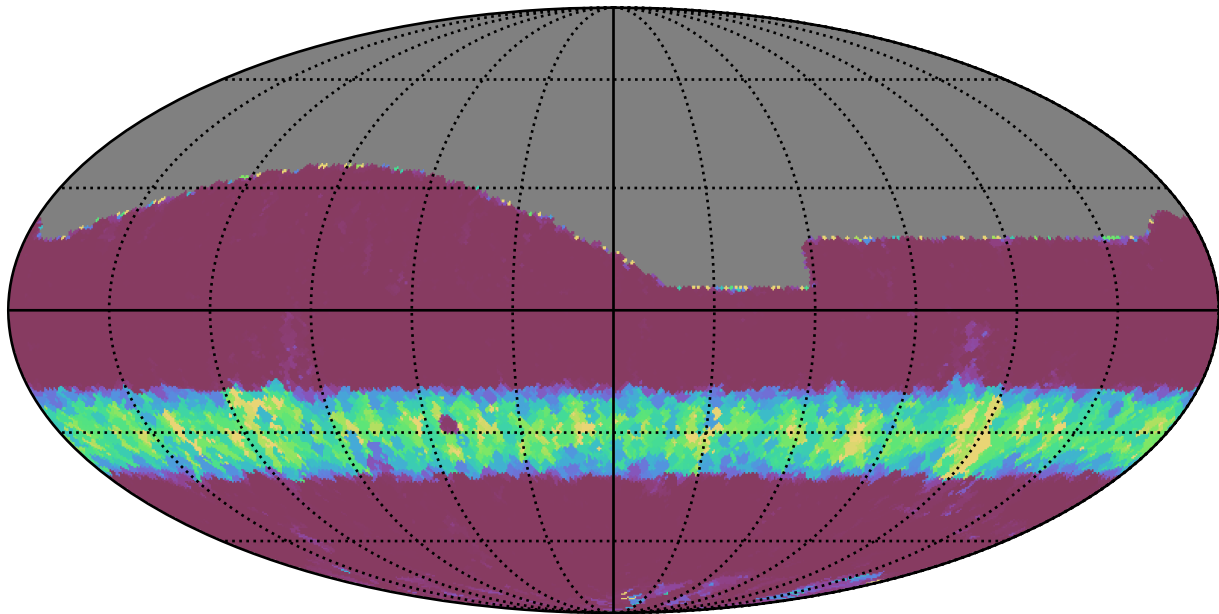
roll_pause_mjdp0_v3.4_10yrs All sky g band: Min normairmass
