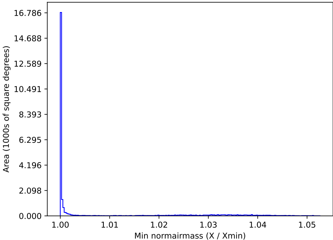
roll_pause_mjdp0_v3.4_10yrs All sky g band: Min normairmass
