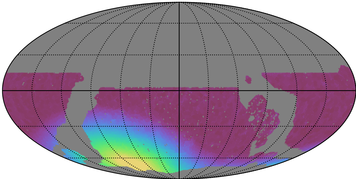
roll_pause_mjdp0_v3.4_10yrs WFD z band: Min moonDistance
