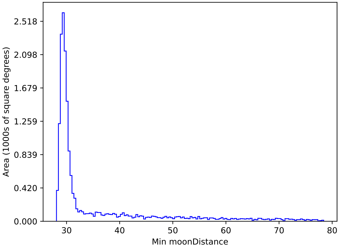
roll_pause_mjdp0_v3.4_10yrs WFD y band: Min moonDistance
