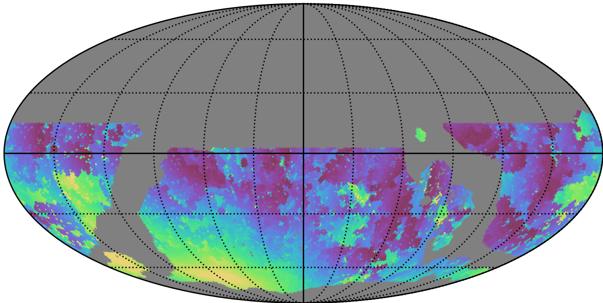
roll_pause_mjdp0_v3.4_10yrs WFD u band: Min moonDistance
