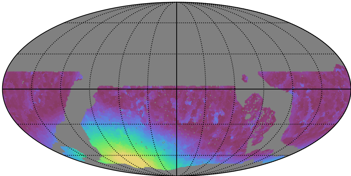
roll_pause_mjdp0_v3.4_10yrs WFD r band: Min moonDistance
