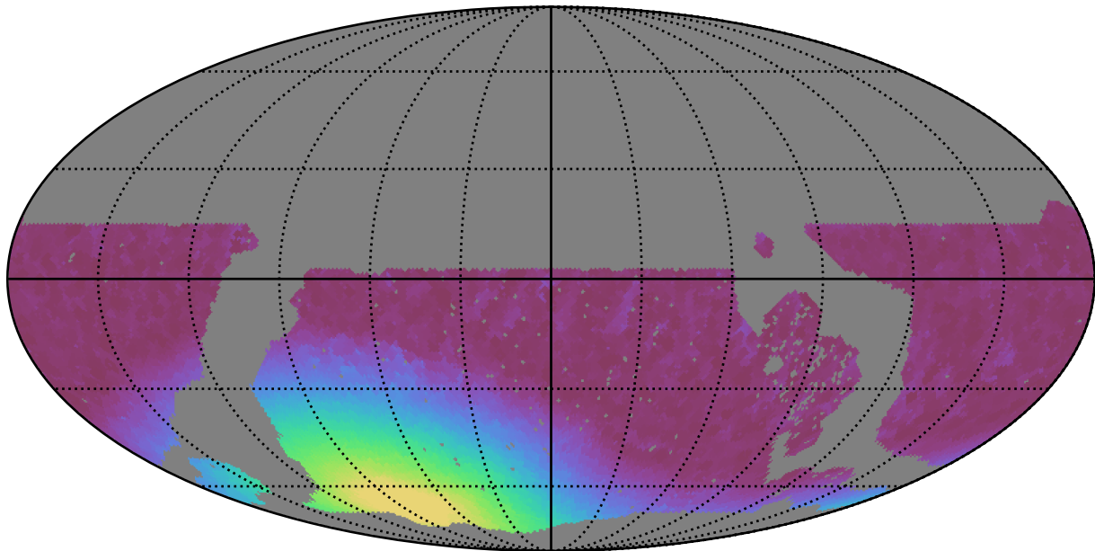
roll_pause_mjdp0_v3.4_10yrs WFD i band: Min moonDistance
