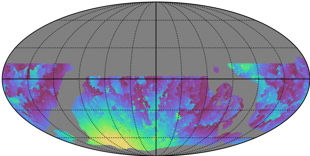
roll_pause_mjdp0_v3.4_10yrs WFD g band: Min moonDistance
