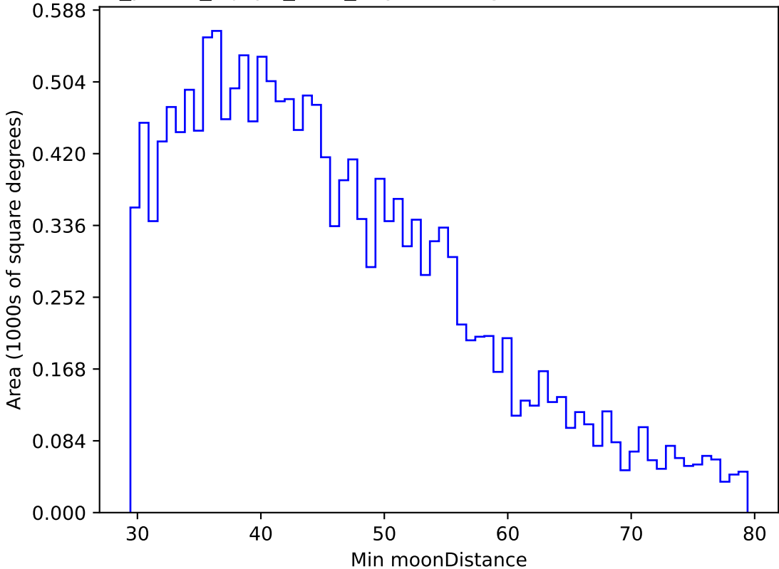
roll_pause_mjdp0_v3.4_10yrs WFD g band: Min moonDistance
