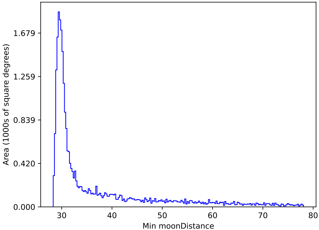
roll_pause_mjdp0_v3.4_10yrs All sky z band: Min moonDistance
