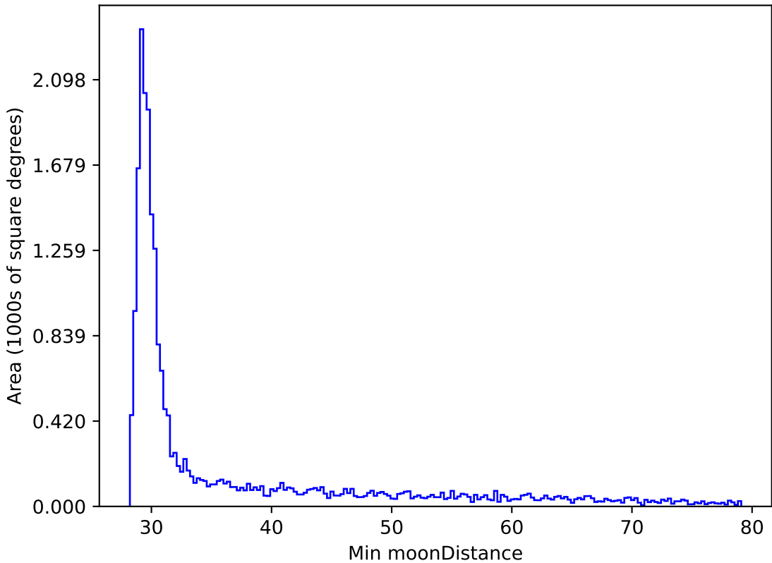
roll_pause_mjdp0_v3.4_10yrs All sky y band: Min moonDistance
