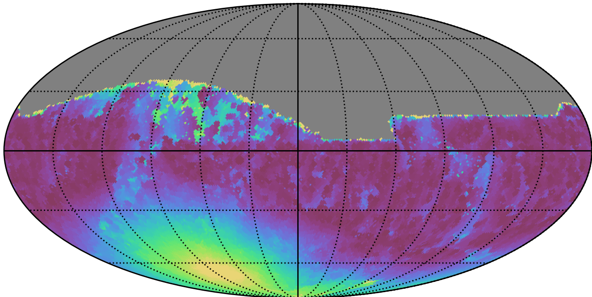
roll_pause_mjdp0_v3.4_10yrs All sky r band: Min moonDistance
