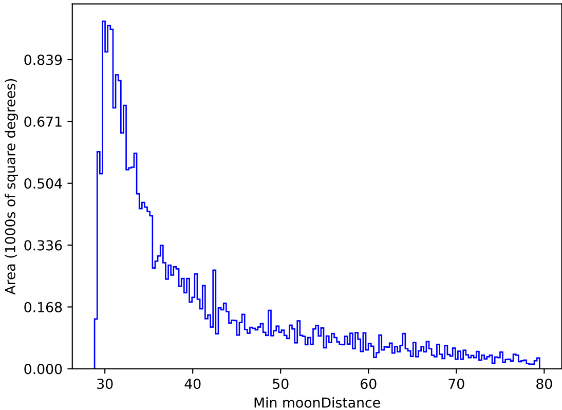
roll_pause_mjdp0_v3.4_10yrs All sky r band: Min moonDistance
