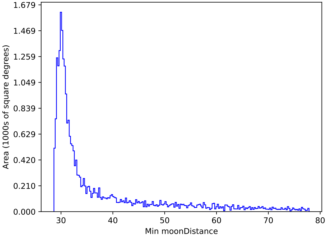
roll_pause_mjdp0_v3.4_10yrs All sky i band: Min moonDistance
