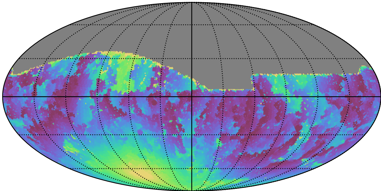
roll_pause_mjdp0_v3.4_10yrs All sky g band: Min moonDistance
