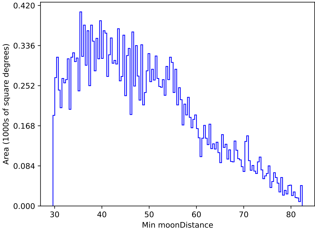
roll_pause_mjdp0_v3.4_10yrs All sky g band: Min moonDistance
