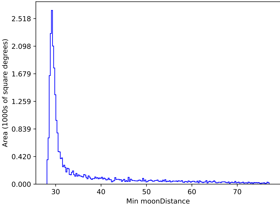
roll_pause_mjdp0_v3.4_10yrs All sky all bands: Min moonDistance
