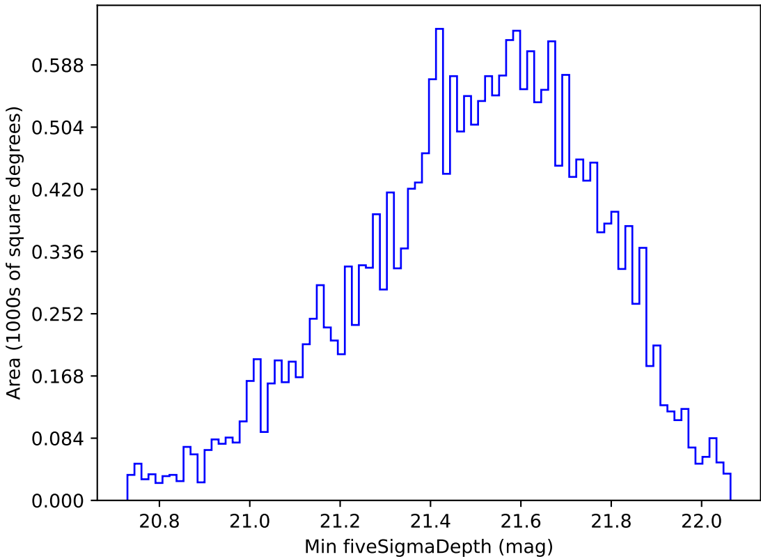
roll_pause_mjdp0_v3.4_10yrs Yr 1 y band: Min fiveSigmaDepth
