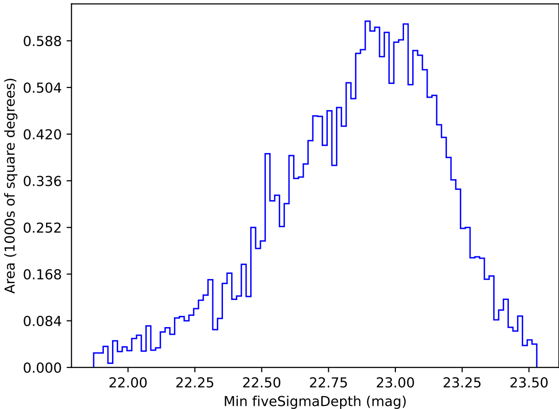
roll_pause_mjdp0_v3.4_10yrs Yr 1 u band: Min fiveSigmaDepth
