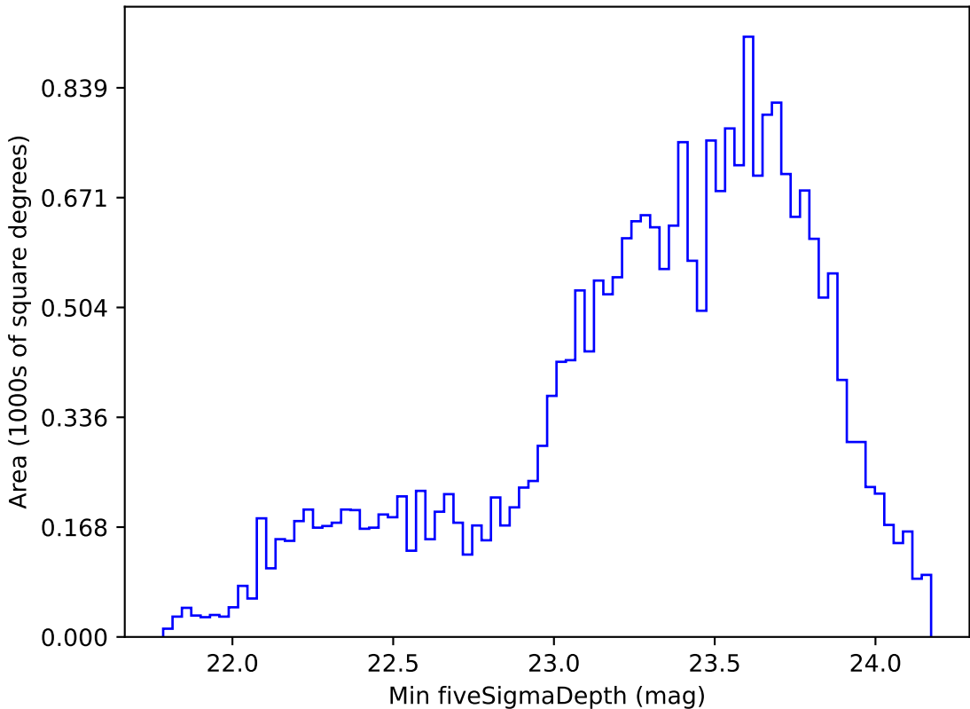
roll_pause_mjdp0_v3.4_10yrs Yr 1 r band: Min fiveSigmaDepth
