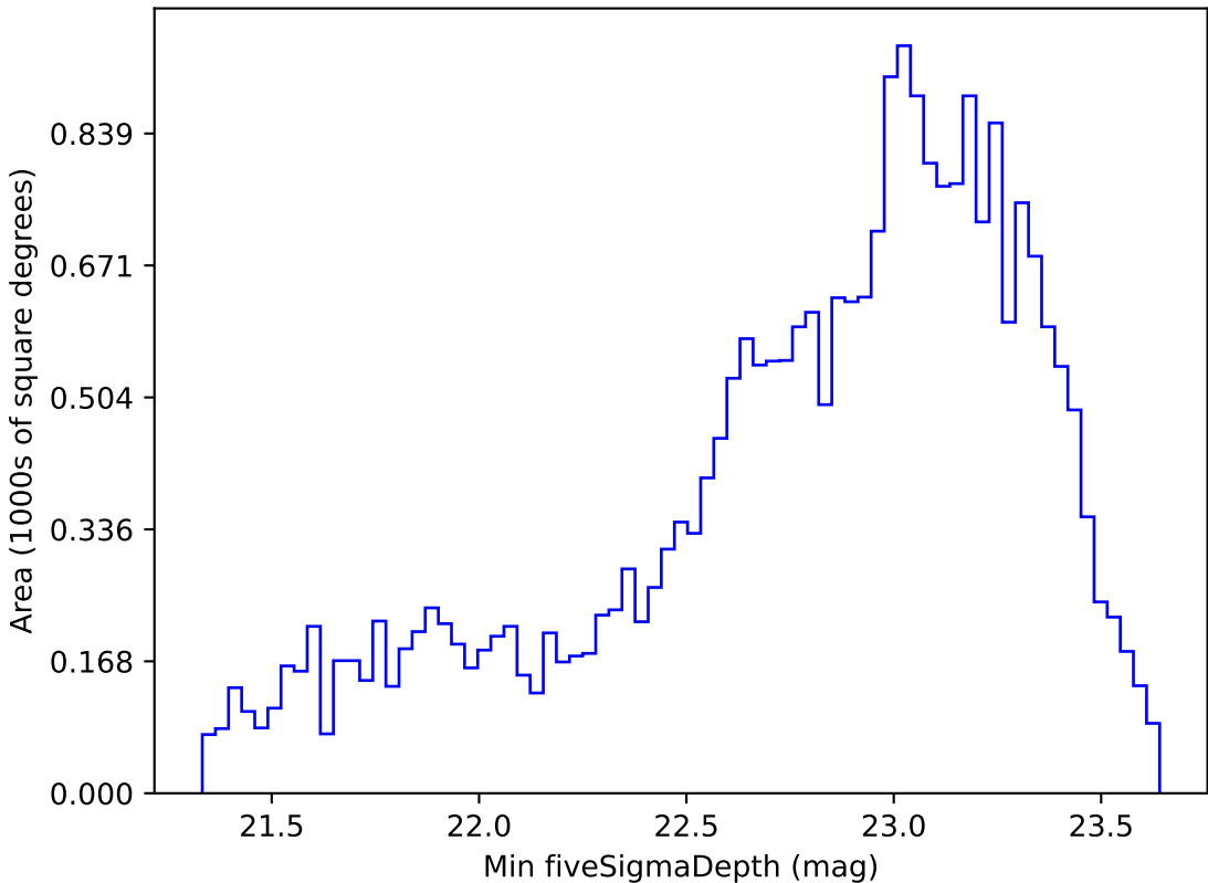
roll_pause_mjdp0_v3.4_10yrs Yr 1 i band: Min fiveSigmaDepth
