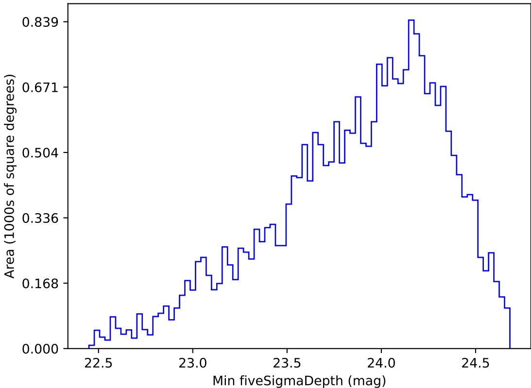
roll_pause_mjdp0_v3.4_10yrs Yr 1 g band: Min fiveSigmaDepth
