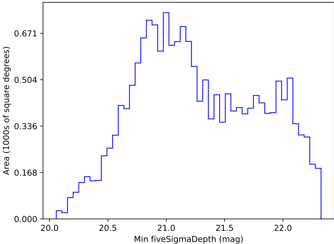
roll_pause_mjdp0_v3.4_10yrs WFD z band: Min fiveSigmaDepth
