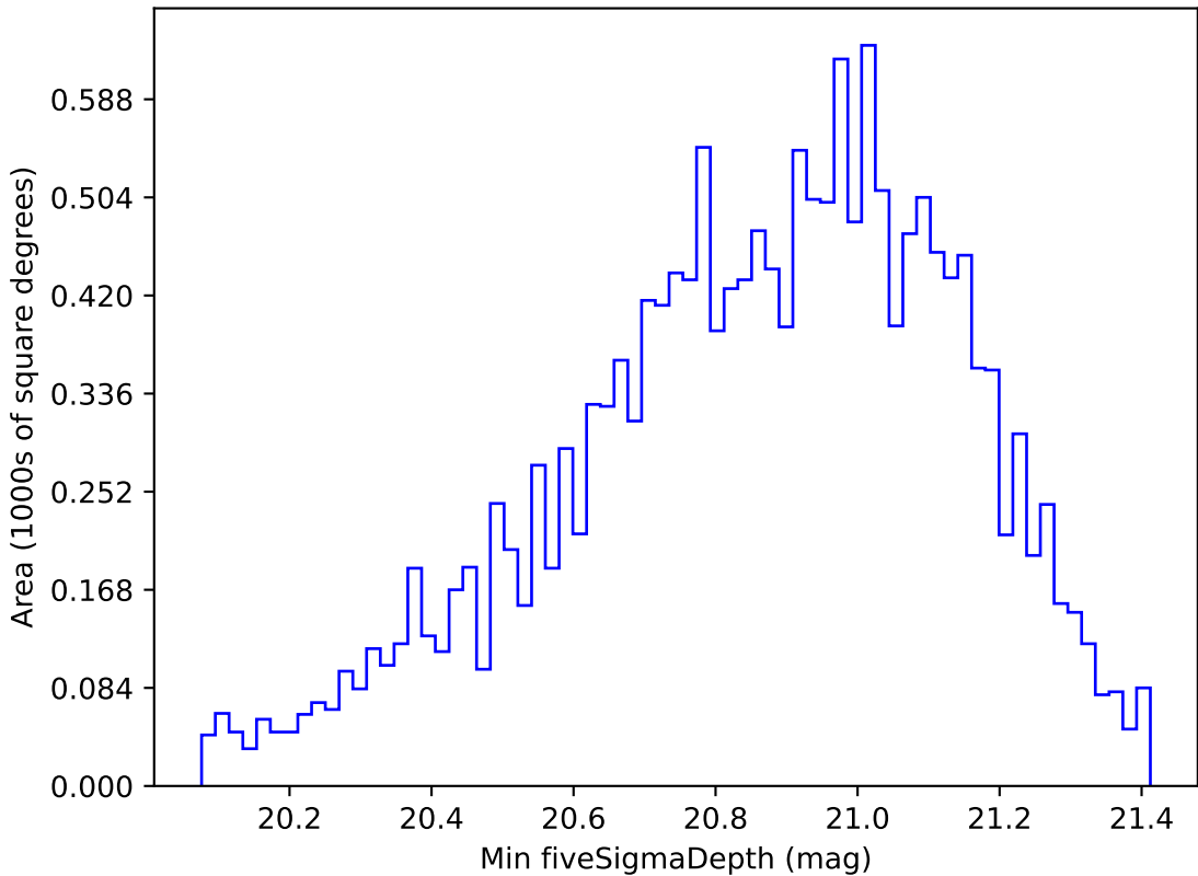
roll_pause_mjdp0_v3.4_10yrs WFD y band: Min fiveSigmaDepth
