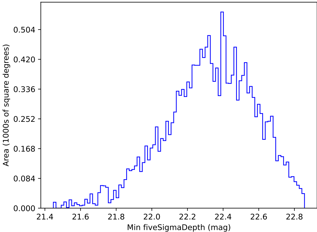
roll_pause_mjdp0_v3.4_10yrs WFD u band: Min fiveSigmaDepth
