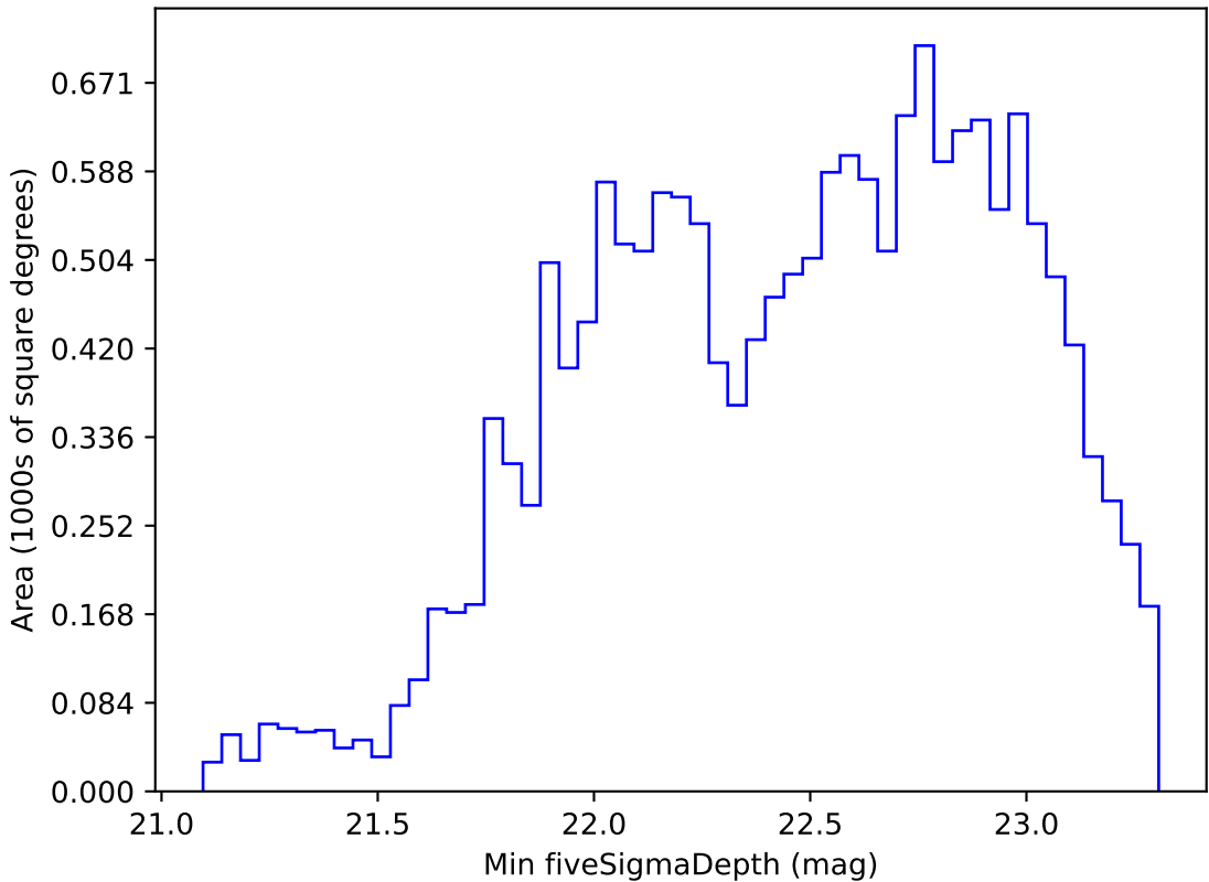
roll_pause_mjdp0_v3.4_10yrs WFD r band: Min fiveSigmaDepth
