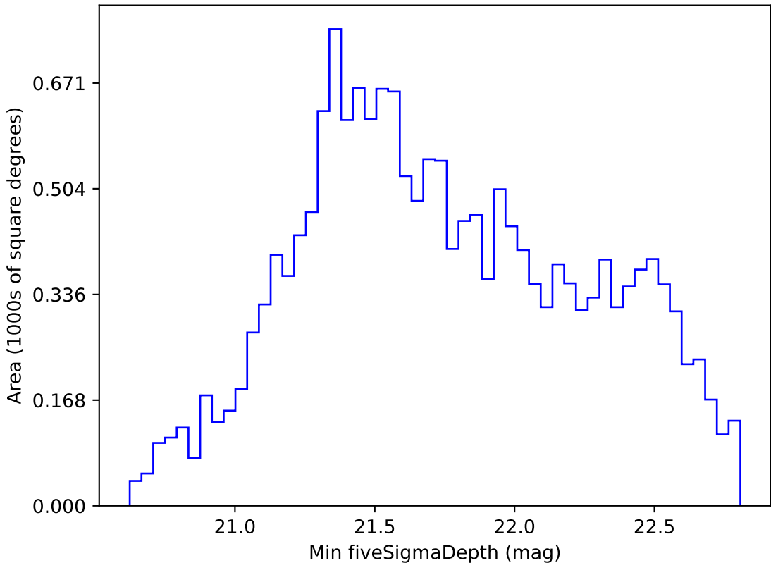
roll_pause_mjdp0_v3.4_10yrs WFD i band: Min fiveSigmaDepth
