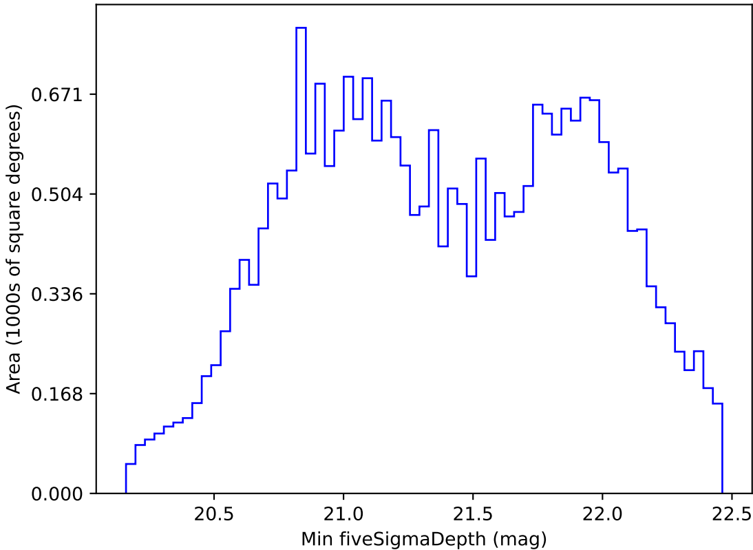
roll_pause_mjdp0_v3.4_10yrs All sky z band: Min fiveSigmaDepth
