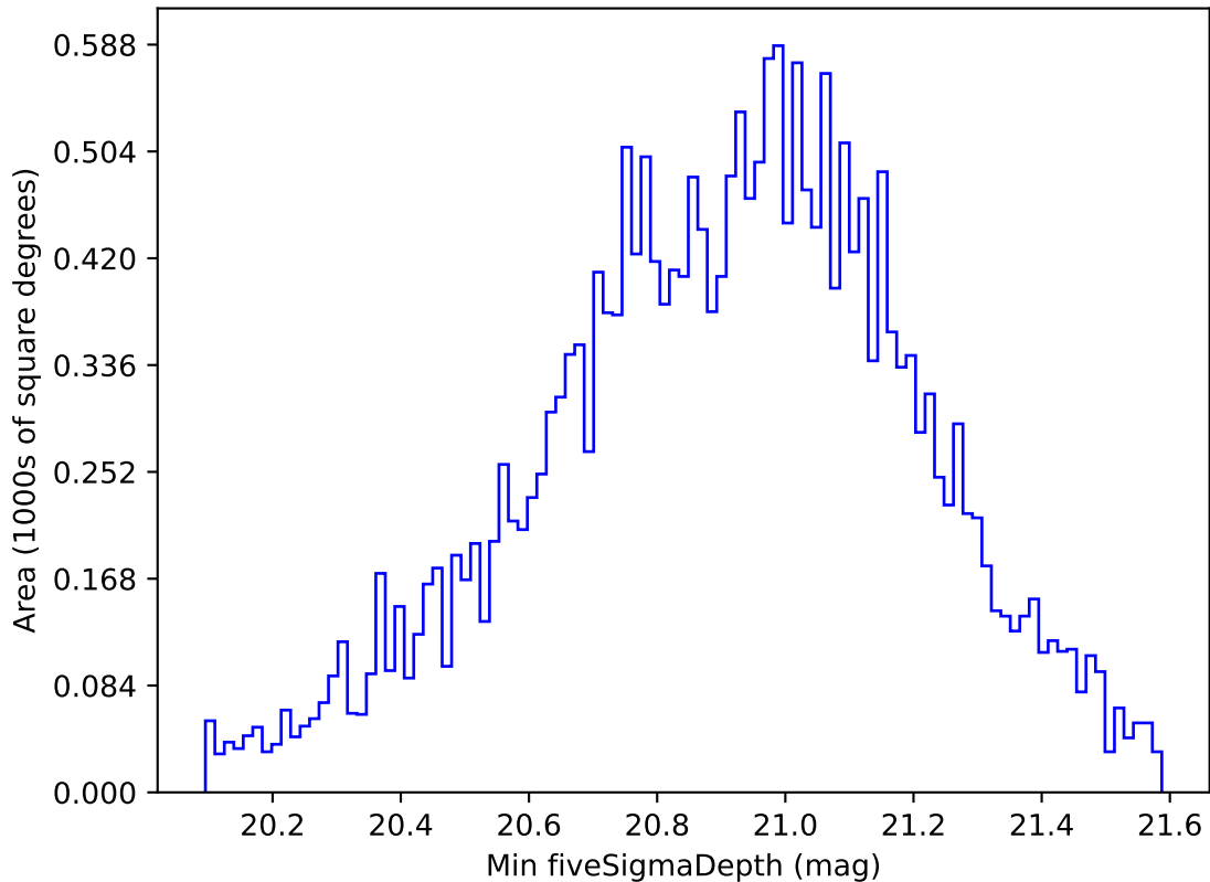
roll_pause_mjdp0_v3.4_10yrs All sky y band: Min fiveSigmaDepth
