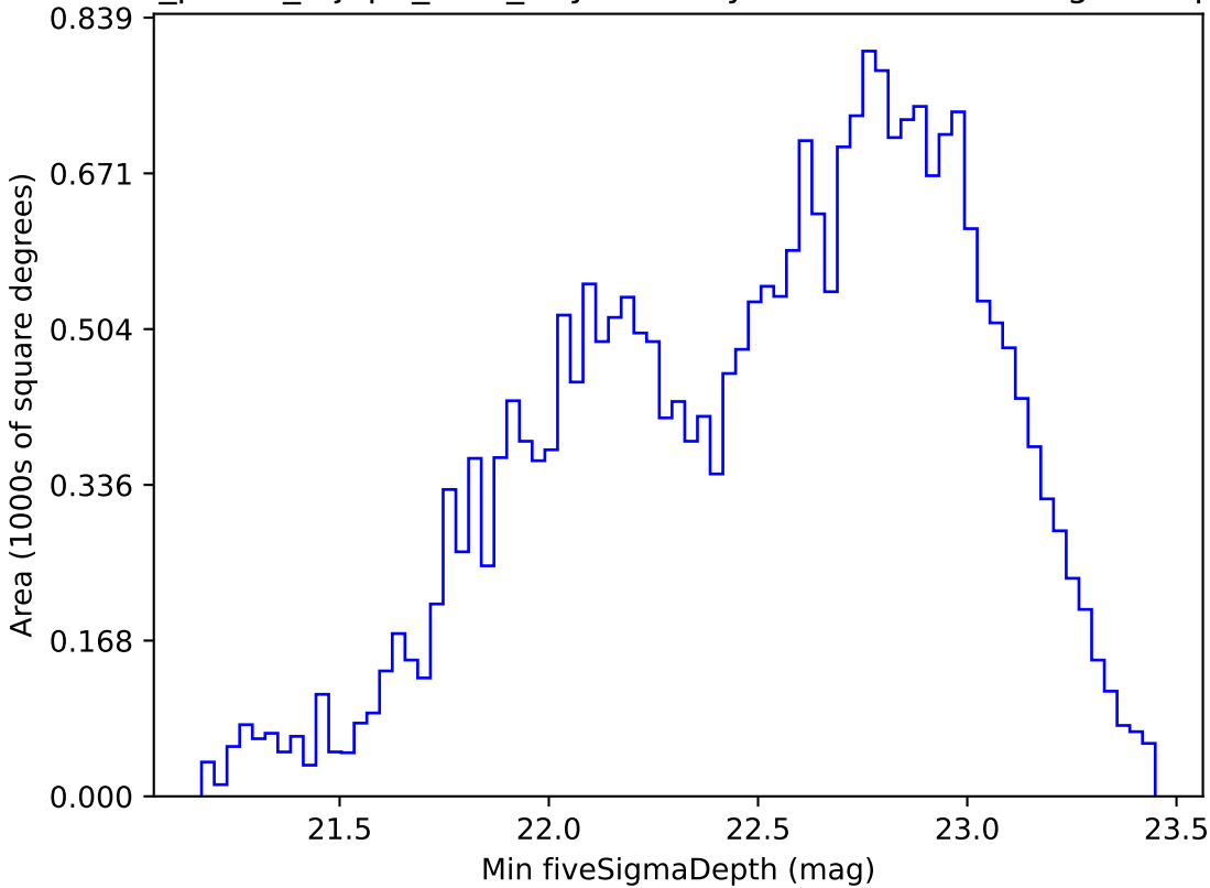
roll_pause_mjdp0_v3.4_10yrs All sky r band: Min fiveSigmaDepth
