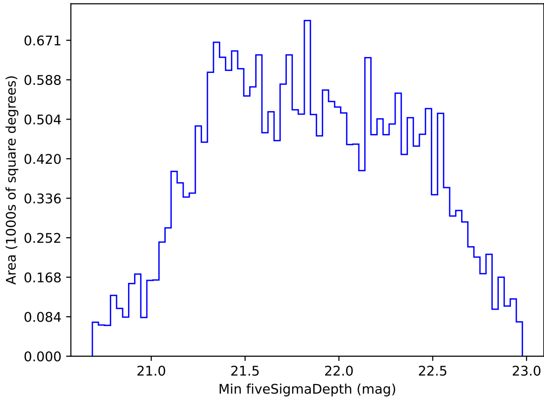
roll_pause_mjdp0_v3.4_10yrs All sky i band: Min fiveSigmaDepth
