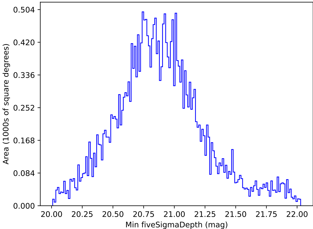
roll_pause_mjdp0_v3.4_10yrs All sky all bands: Min fiveSigmaDepth
