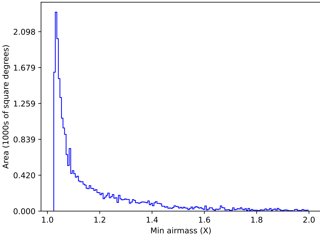
roll_pause_mjdp0_v3.4_10yrs Yr 1 z band: Min airmass
