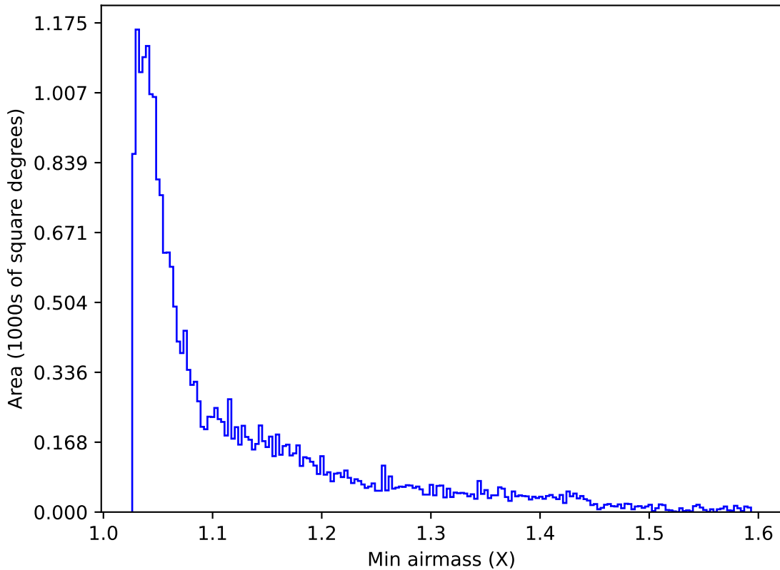
roll_pause_mjdp0_v3.4_10yrs Yr 1 y band: Min airmass
