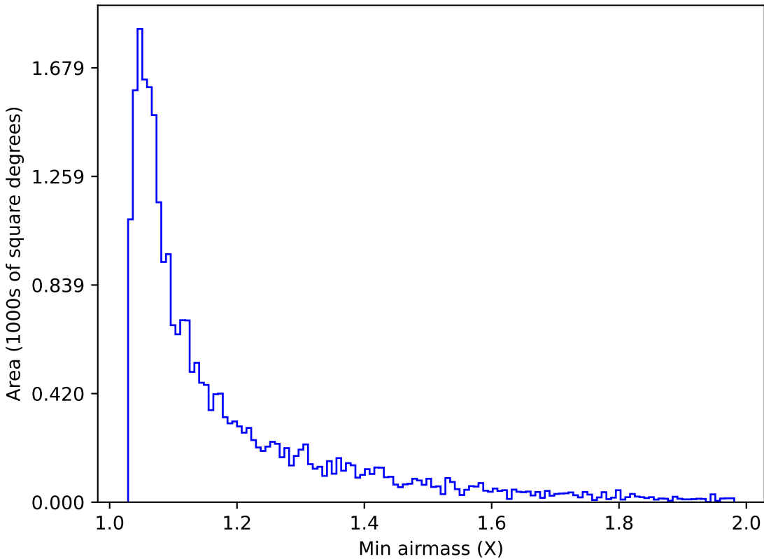
roll_pause_mjdp0_v3.4_10yrs Yr 1 g band: Min airmass
