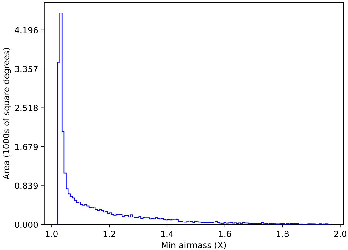
roll_pause_mjdp0_v3.4_10yrs Yr 1 all bands: Min airmass
