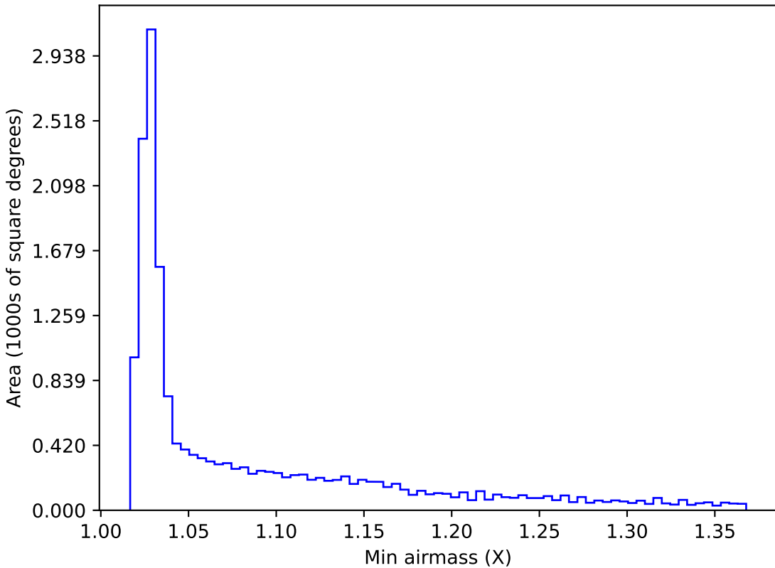
roll_pause_mjdp0_v3.4_10yrs WFD r band: Min airmass
