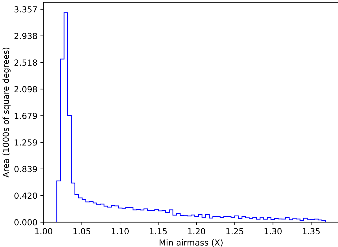
roll_pause_mjdp0_v3.4_10yrs WFD i band: Min airmass
