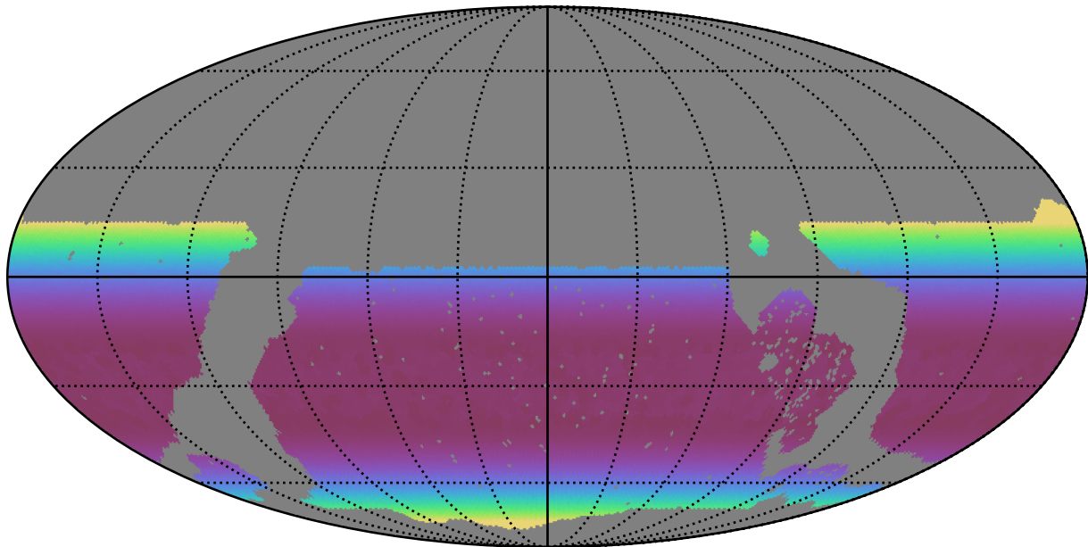
roll_pause_mjdp0_v3.4_10yrs WFD all bands: Min airmass
