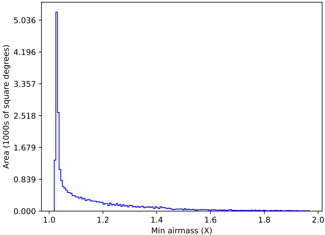
roll_pause_mjdp0_v3.4_10yrs All sky z band: Min airmass
