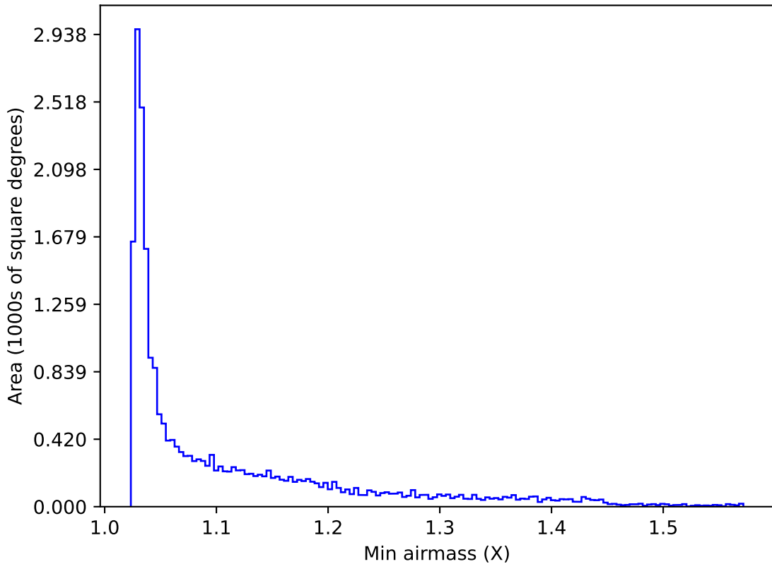
roll_pause_mjdp0_v3.4_10yrs All sky y band: Min airmass
