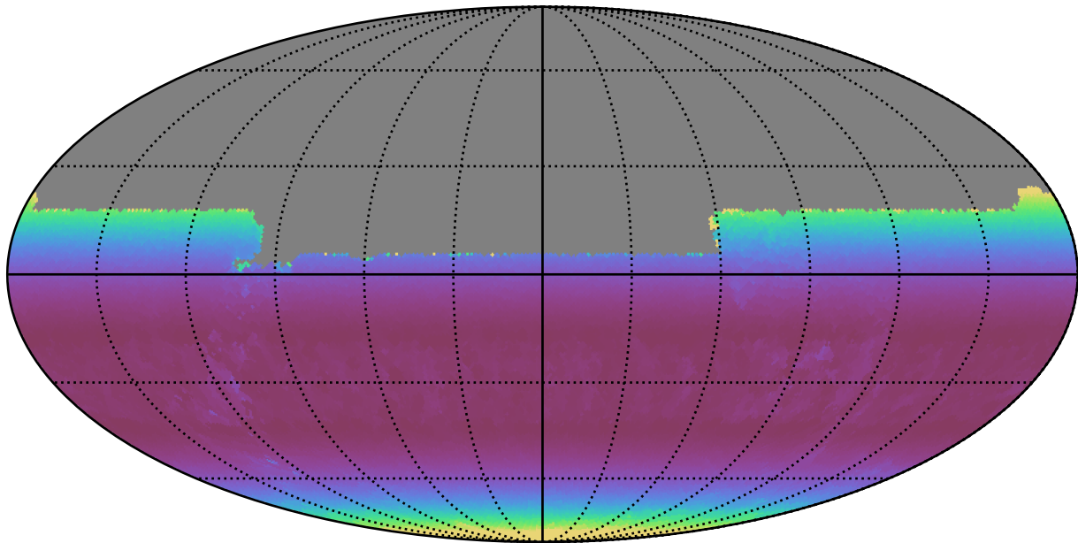
roll_pause_mjdp0_v3.4_10yrs All sky u band: Min airmass
