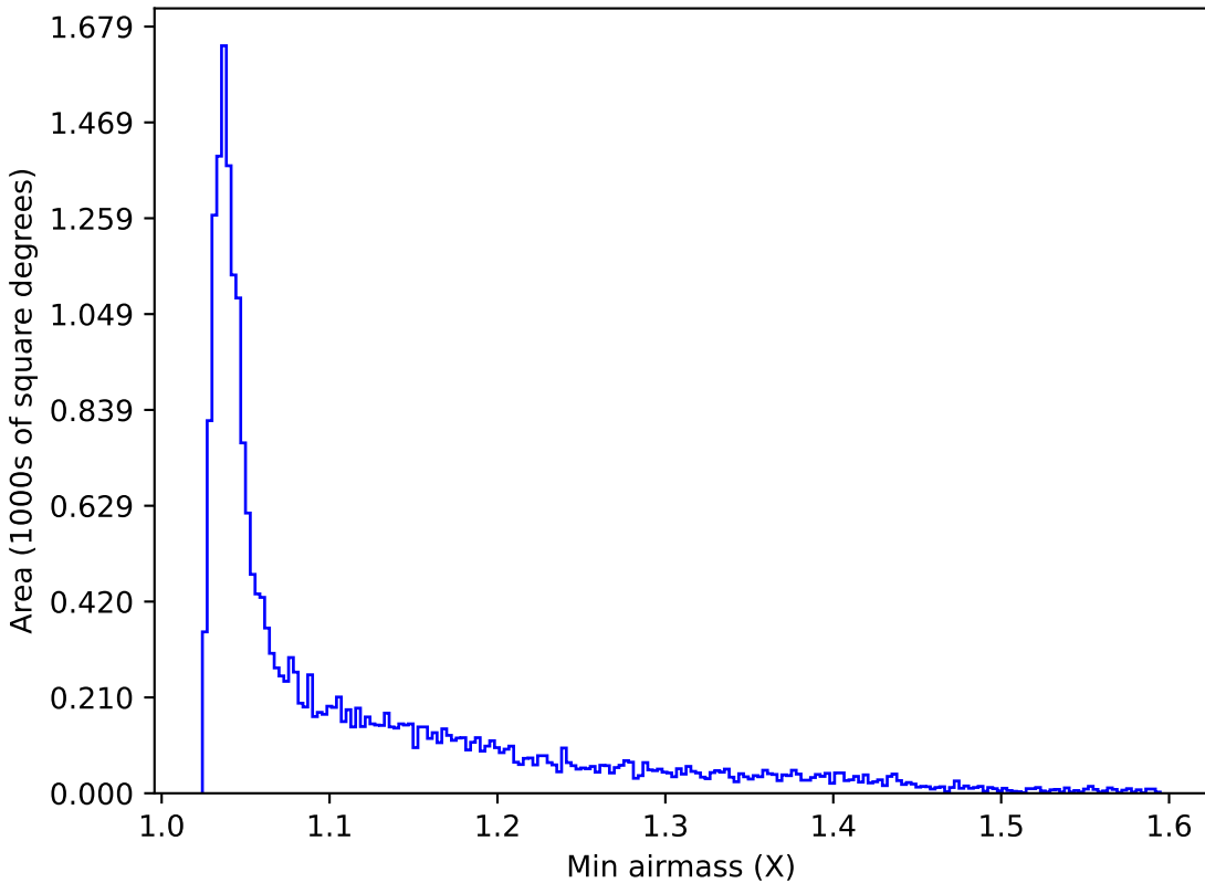
roll_pause_mjdp0_v3.4_10yrs All sky u band: Min airmass
