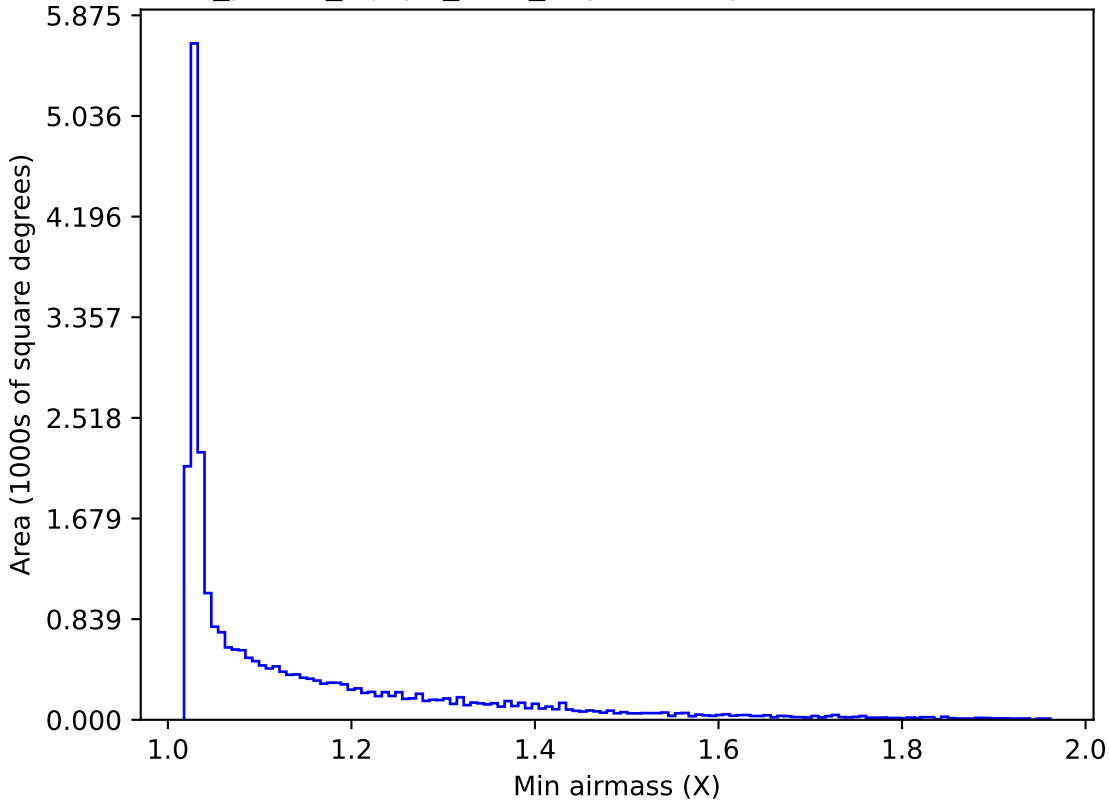
roll_pause_mjdp0_v3.4_10yrs All sky i band: Min airmass
